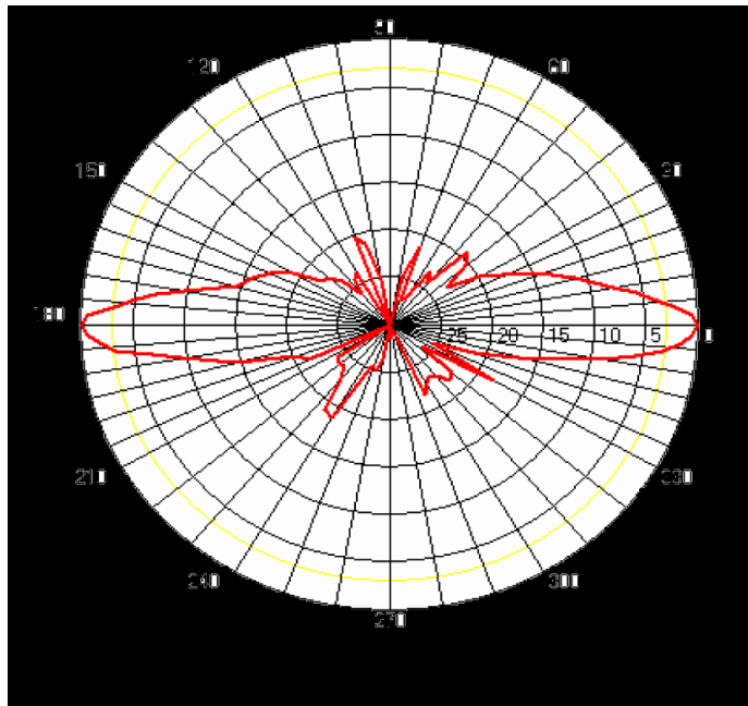
RF Patterns Horizontal Cut
